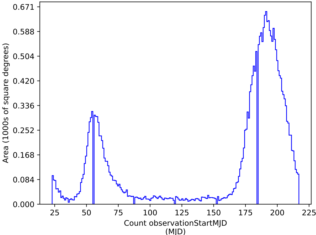
ddf_acor_sf10_lsf20_lsr50_v3.4_10yrs i: Count observationStartMJD
