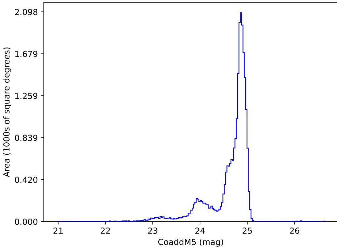
ddf_acor_sf10_lsf20_lsr50_v3.4_10yrs y: CoaddM5
