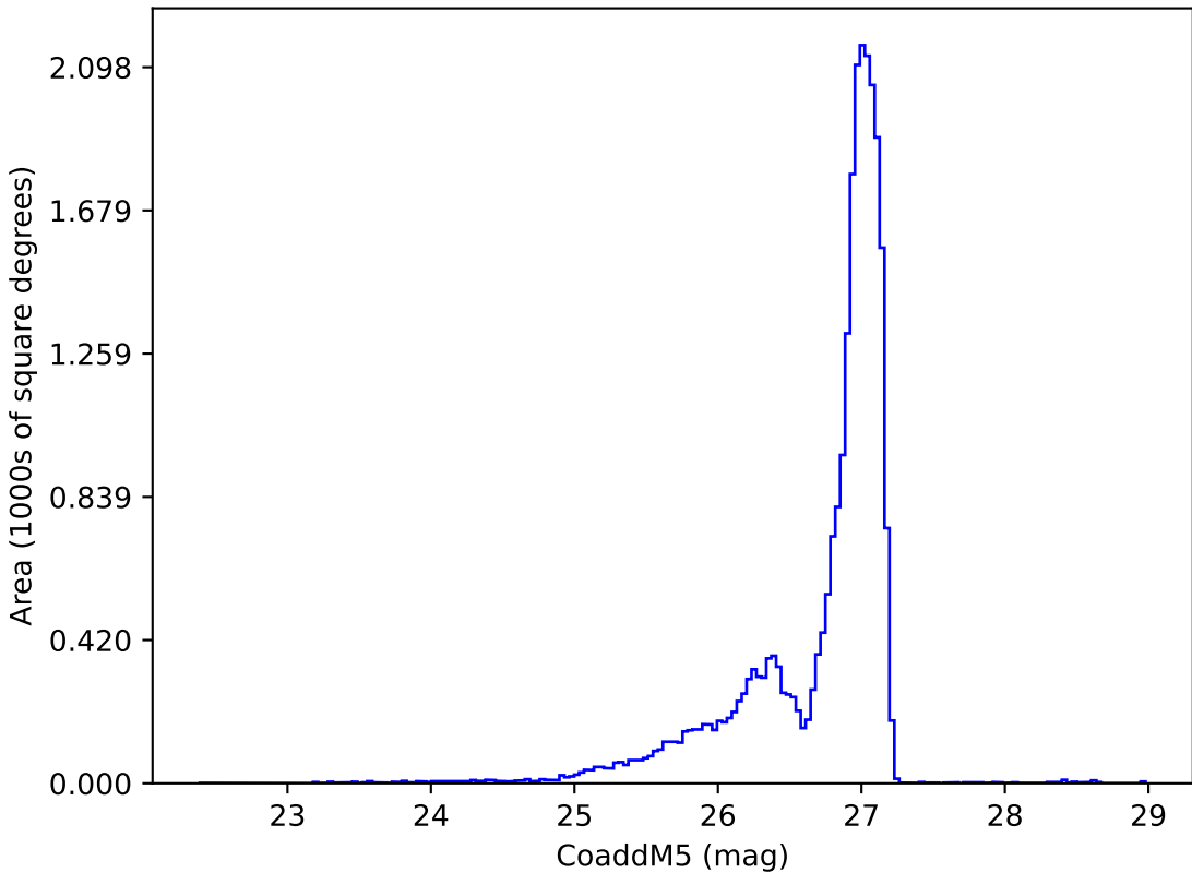
ddf_acor_sf10_lsf20_lsr50_v3.4_10yrs r: CoaddM5
