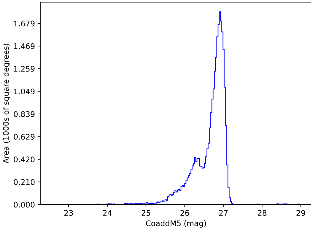
ddf_acor_sf10_lsf20_lsr50_v3.4_10yrs g: CoaddM5
