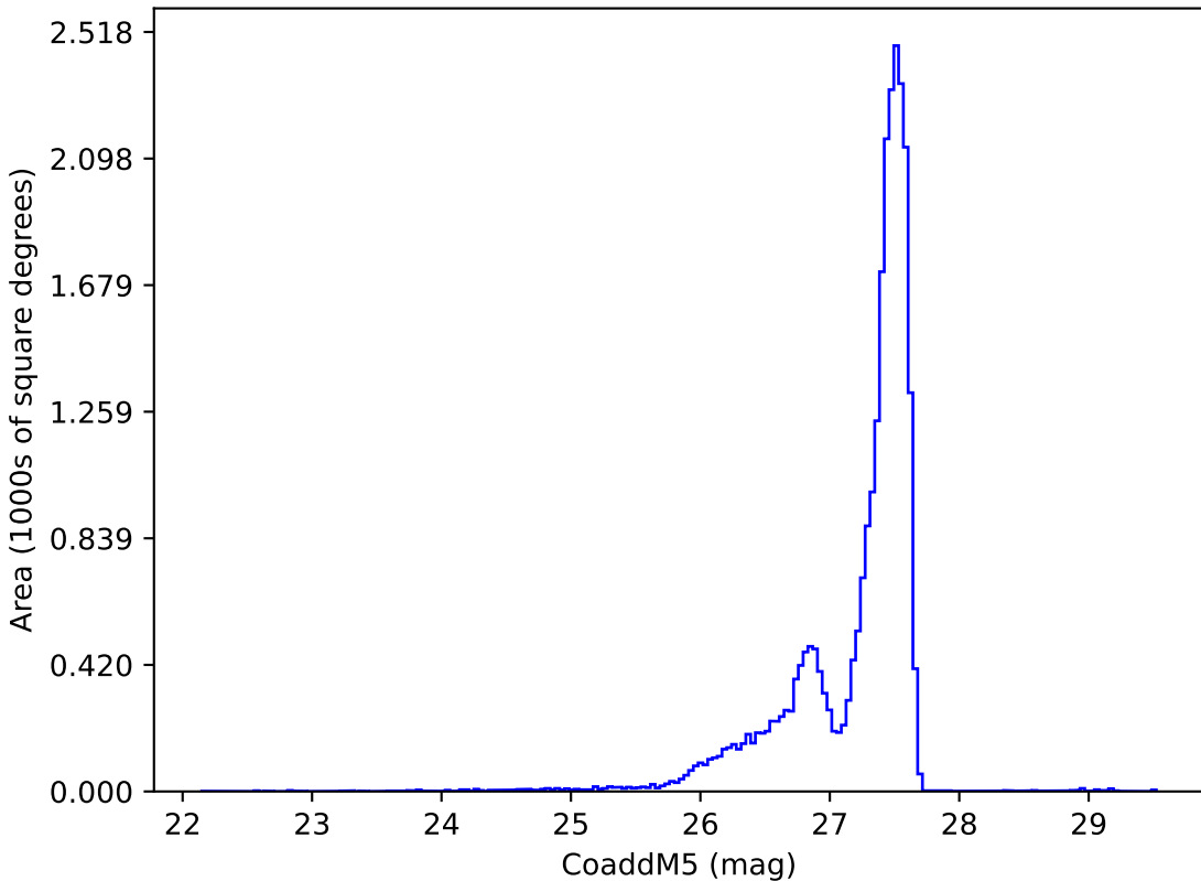
ddf_acor_sf10_lsf20_lsr50_v3.4_10yrs : CoaddM5
