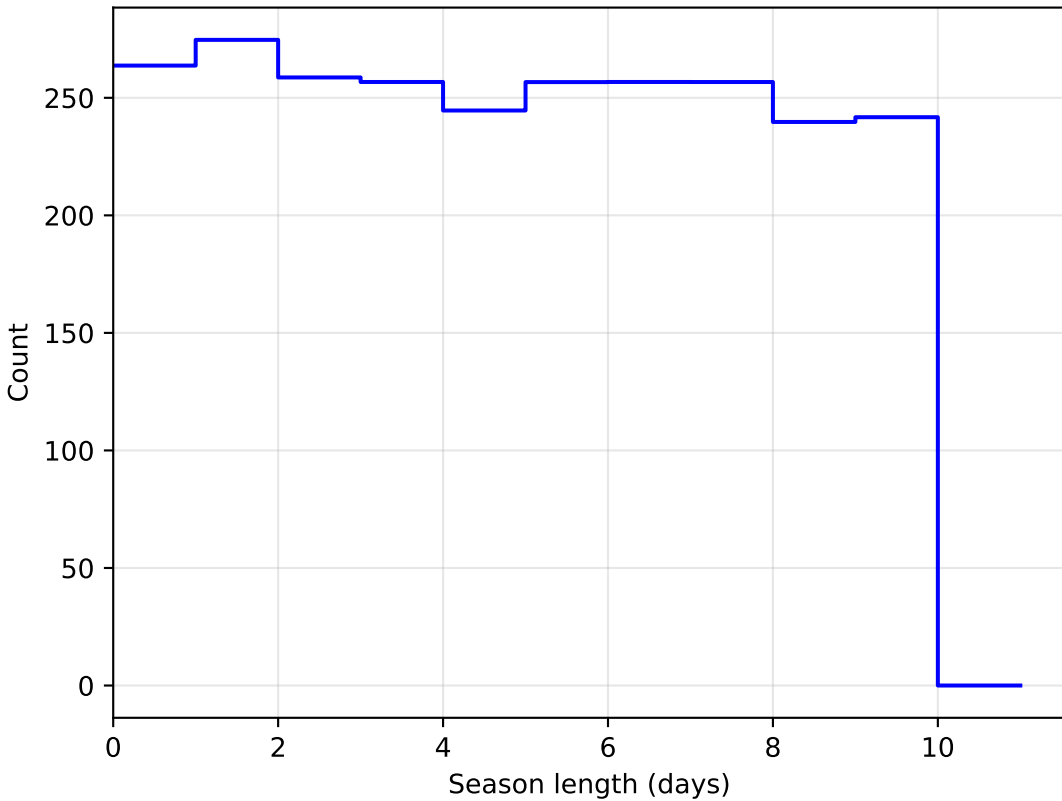
ddf_acor_sf10_lsf20_lsr50_v3.4_10yrs DD:EDFS all bands: SeasonLength
