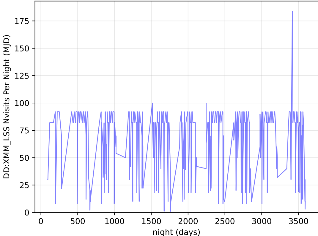
ddf_acor_sf10_lsf20_lsr50_v3.4_10yrs all bands: DD:XMM_LSS Nvisits Per Night
