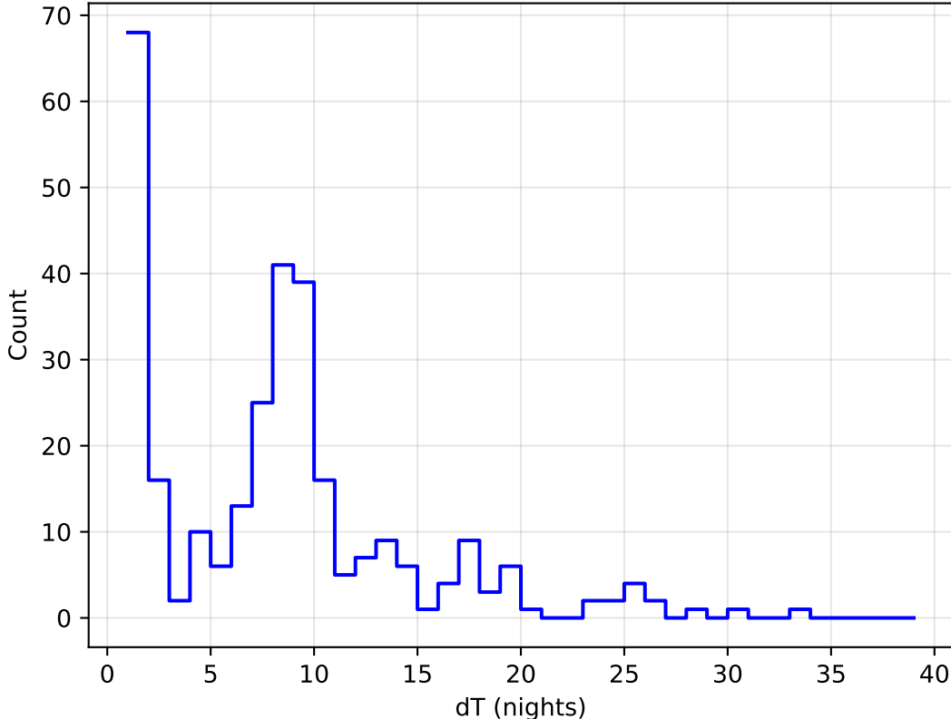
ddf_acor_sf10_Isf20_Isr50_v3.4_10yrs all bands: DD:XMM_LSS Delta Nights Histogram
