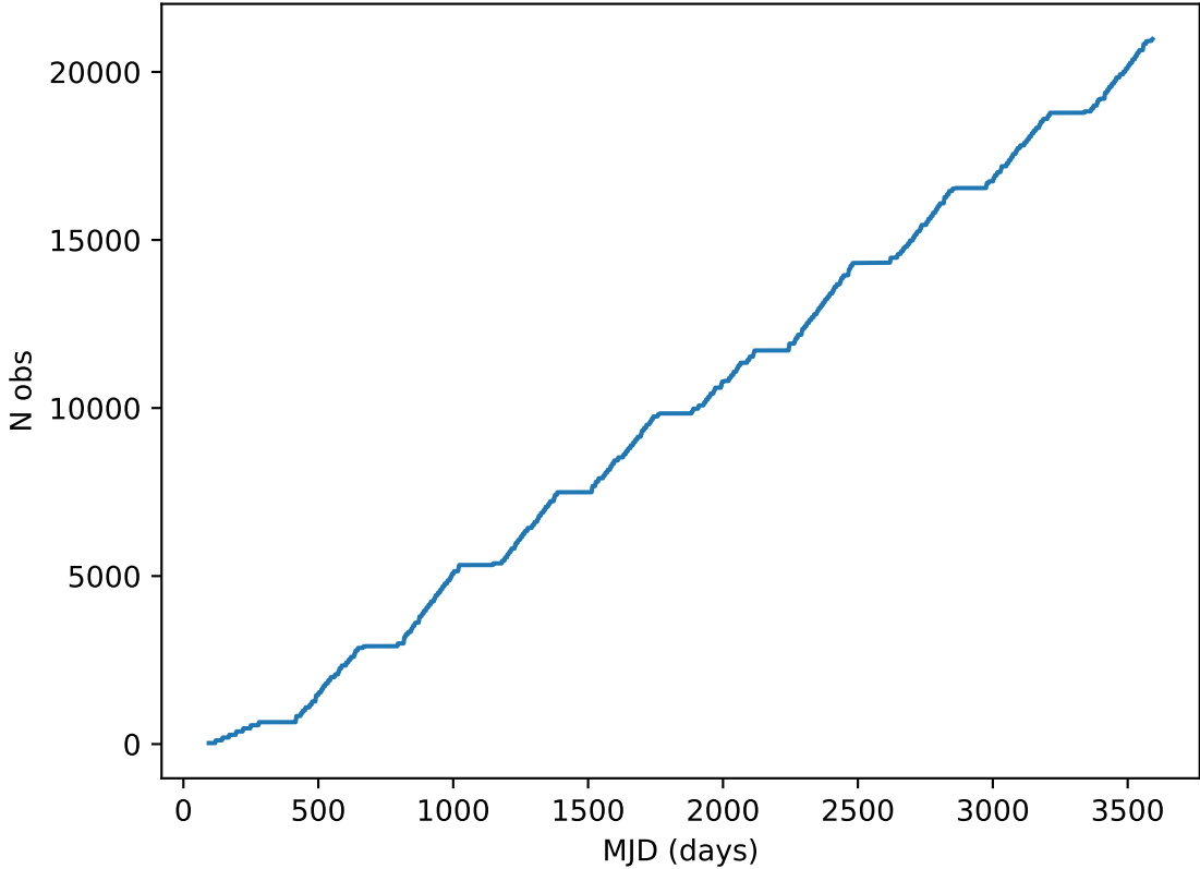
ddf_acor_sf10_lsf20_lsr50_v3.4_10yrs all bands: DD:XMM_LSS Cumulative NVisits
