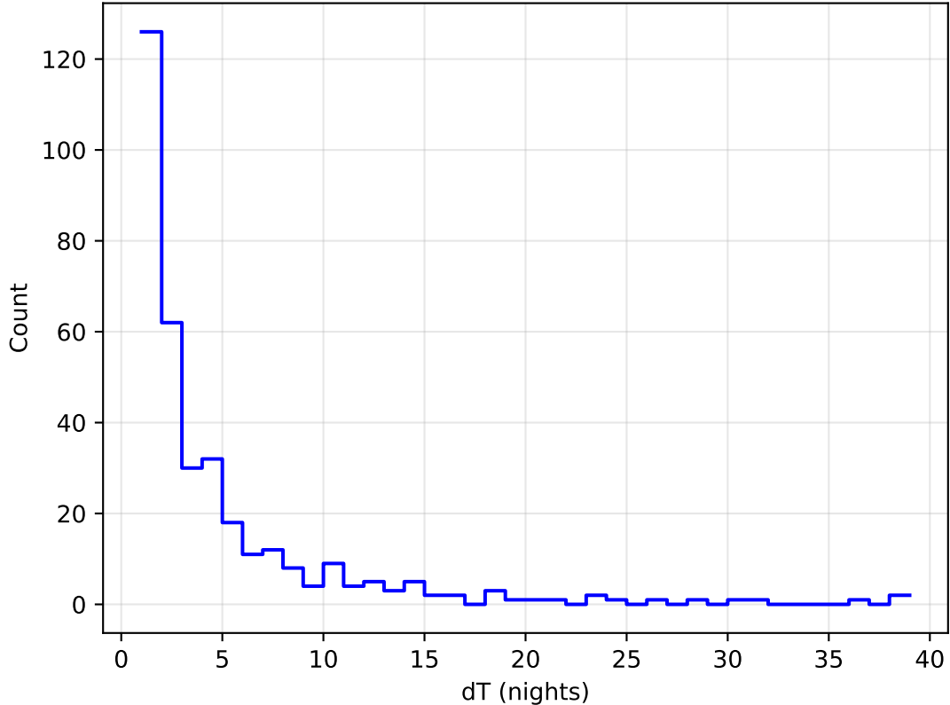
ddf_acor_sf10_lsf20_lsr50_v3.4_10yrs all bands: DD:WFD Delta Nights Histogram
