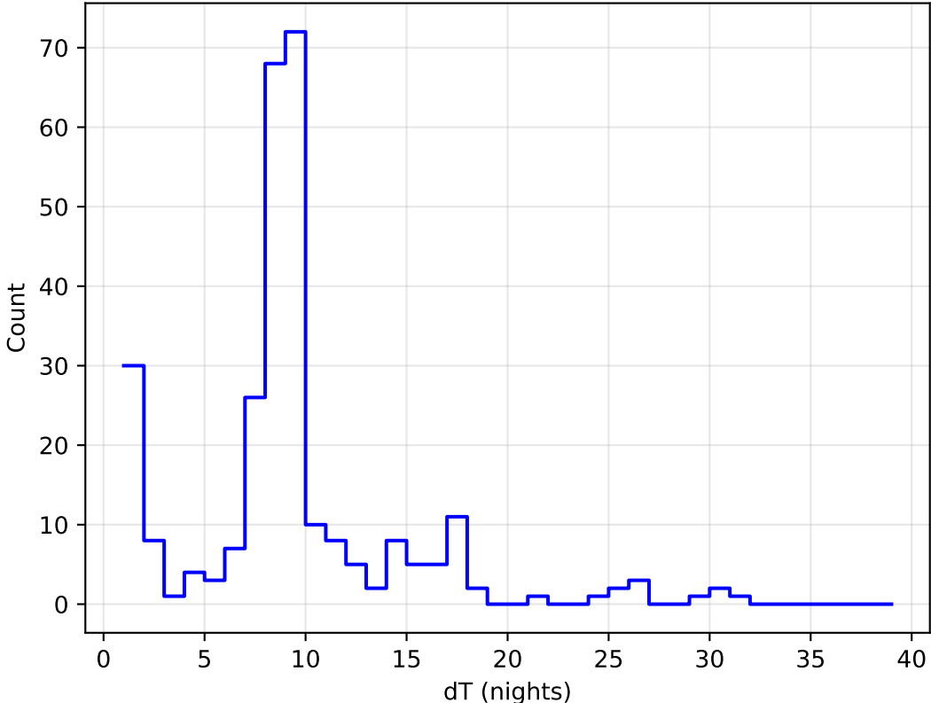
ddf_acor_sf10_lsf20_lsr50_v3.4_10yrs all bands: DD:EDFS Delta Nights Histogram
