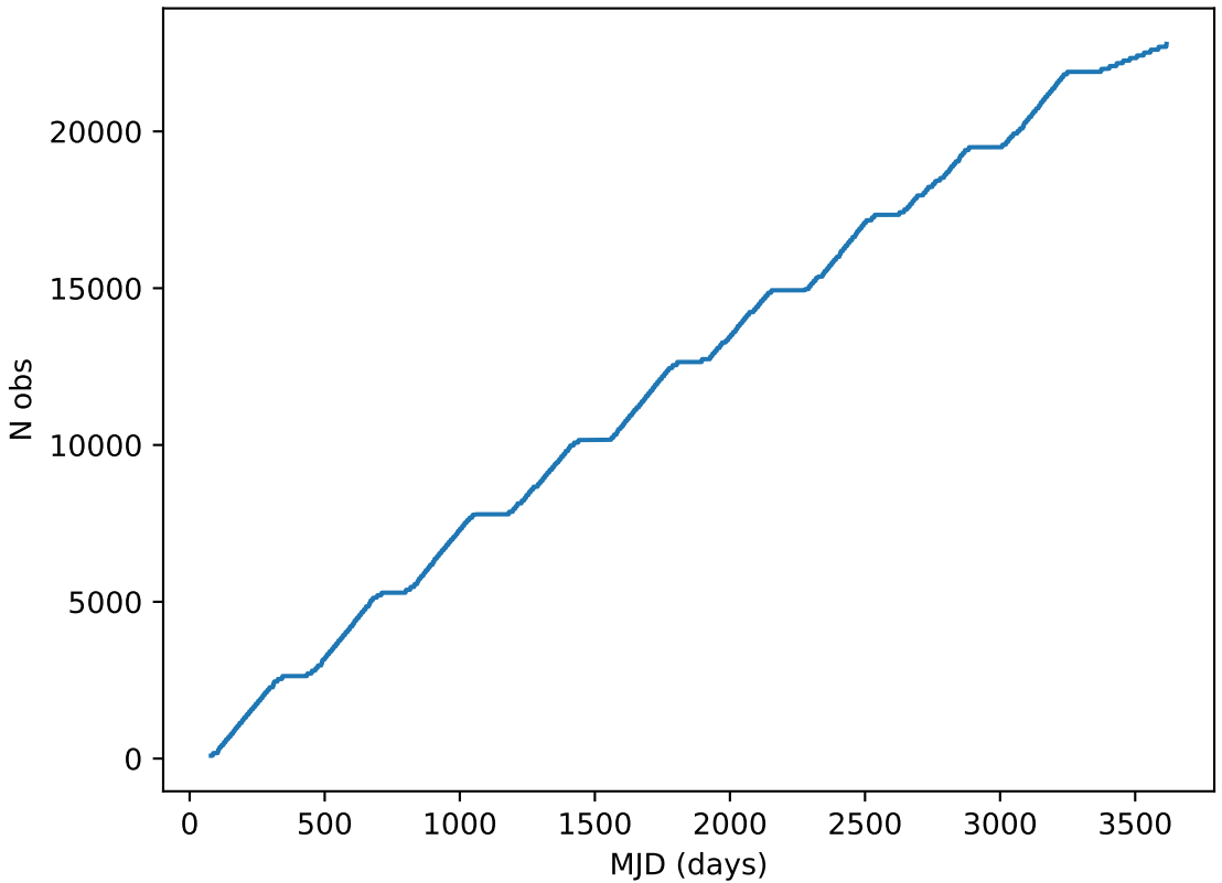
ddf_acor_sf10_lsf20_lsr50_v3.4_10yrs all bands: DD:EDFS Cumulative NVisits
