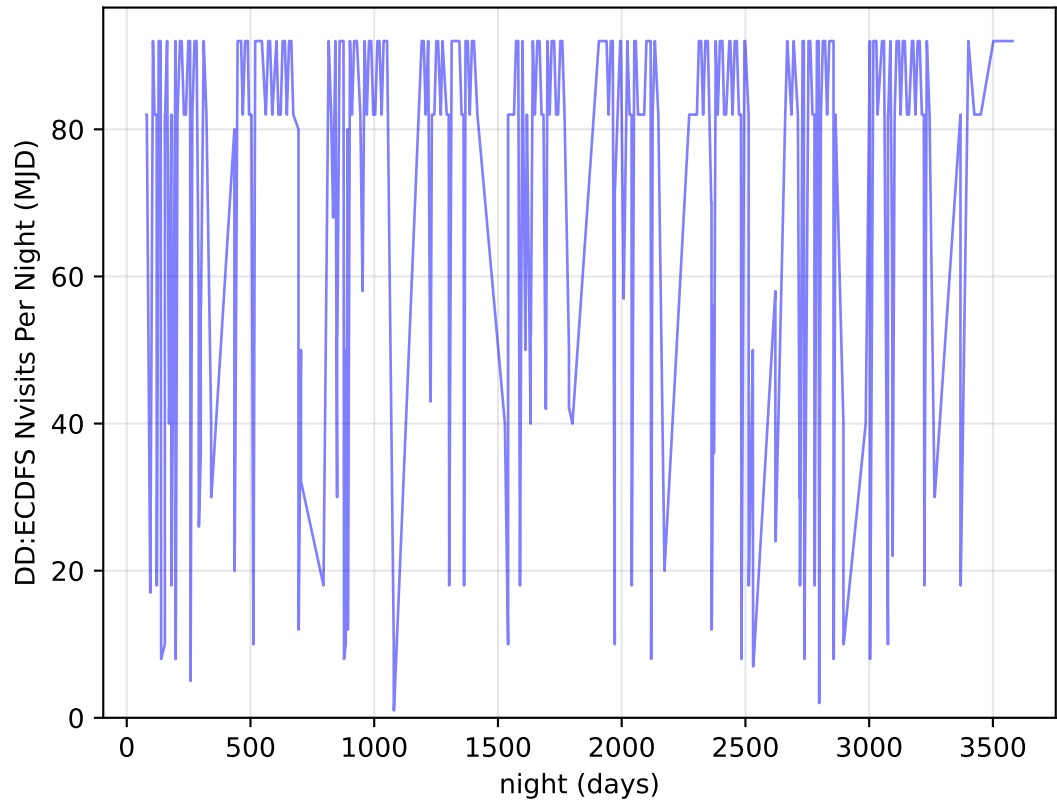
ddf_acor_sf10_lsf20_lsr50_v3.4_10yrs all bands: DD:ECDFS Nvisits Per Night
