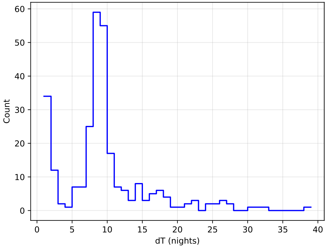
ddf_acor_sf10_lsf20_lsr50_v3.4_10yrs all bands: DD:ECDFS Delta Nights Histogram
