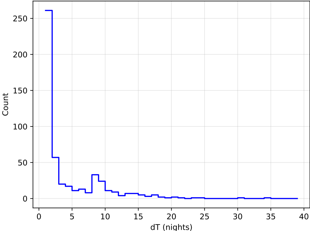
ddf_acor_sf10_lsf20_lsr50_v3.4_10yrs all bands: DD:COSMOS Delta Nights Histogram
