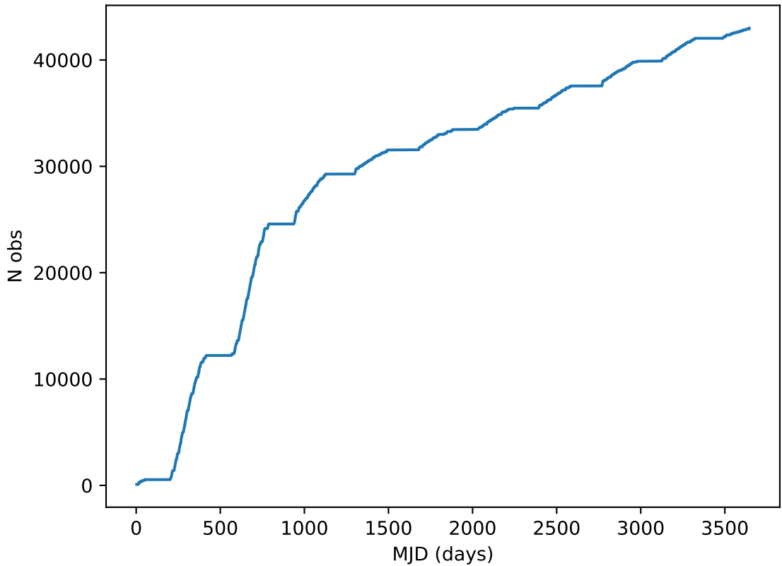
ddf_acor_sf10_lsf20_lsr50_v3.4_10yrs all bands: DD: COSMOS Cumulative NVisits
