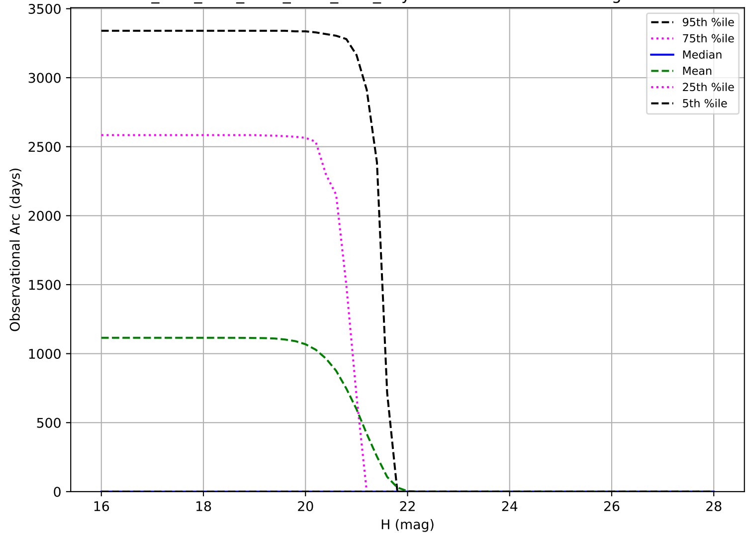
ddf_acor_sf10_lsf20_lsr20_v3.4_10yrs: Observational Arc Length Vatira
