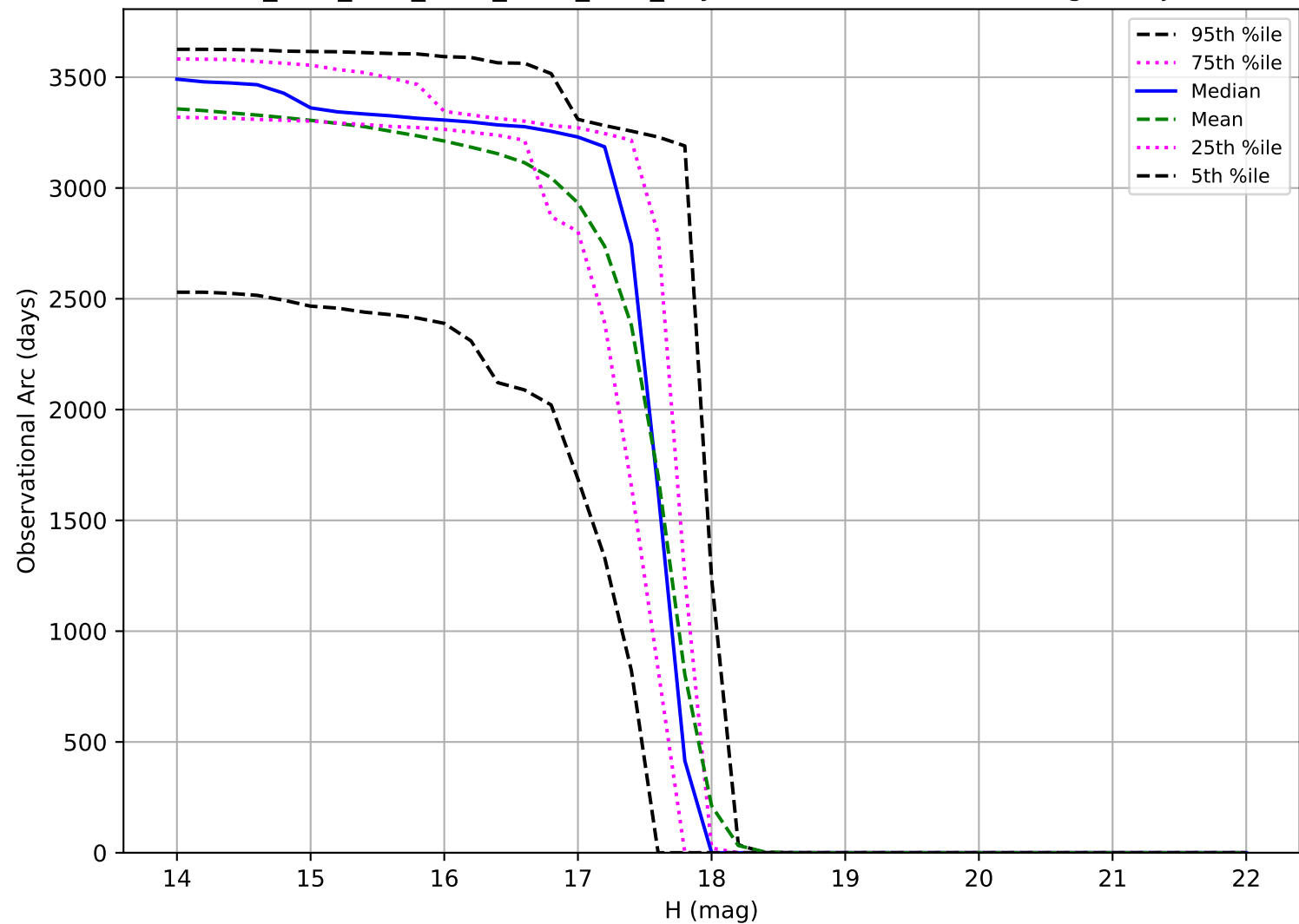
ddf_acor_sf10_lsf20_lsr20_v3.4_10yrs: Observational Arc Length Trojan
