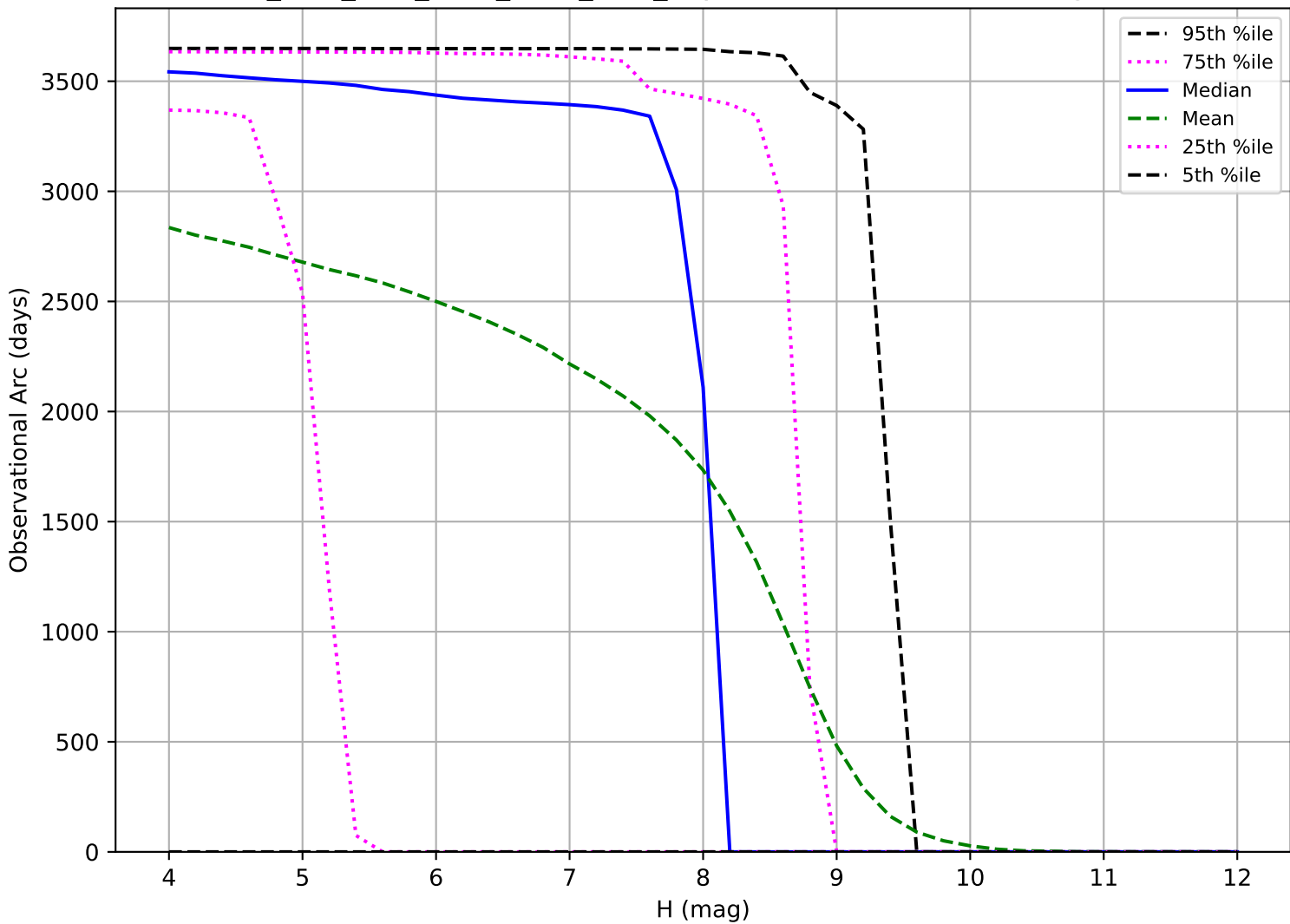
ddf_acor_sf10_lsf20_lsr20_v3.4_10yrs: Observational Arc Length TNO
