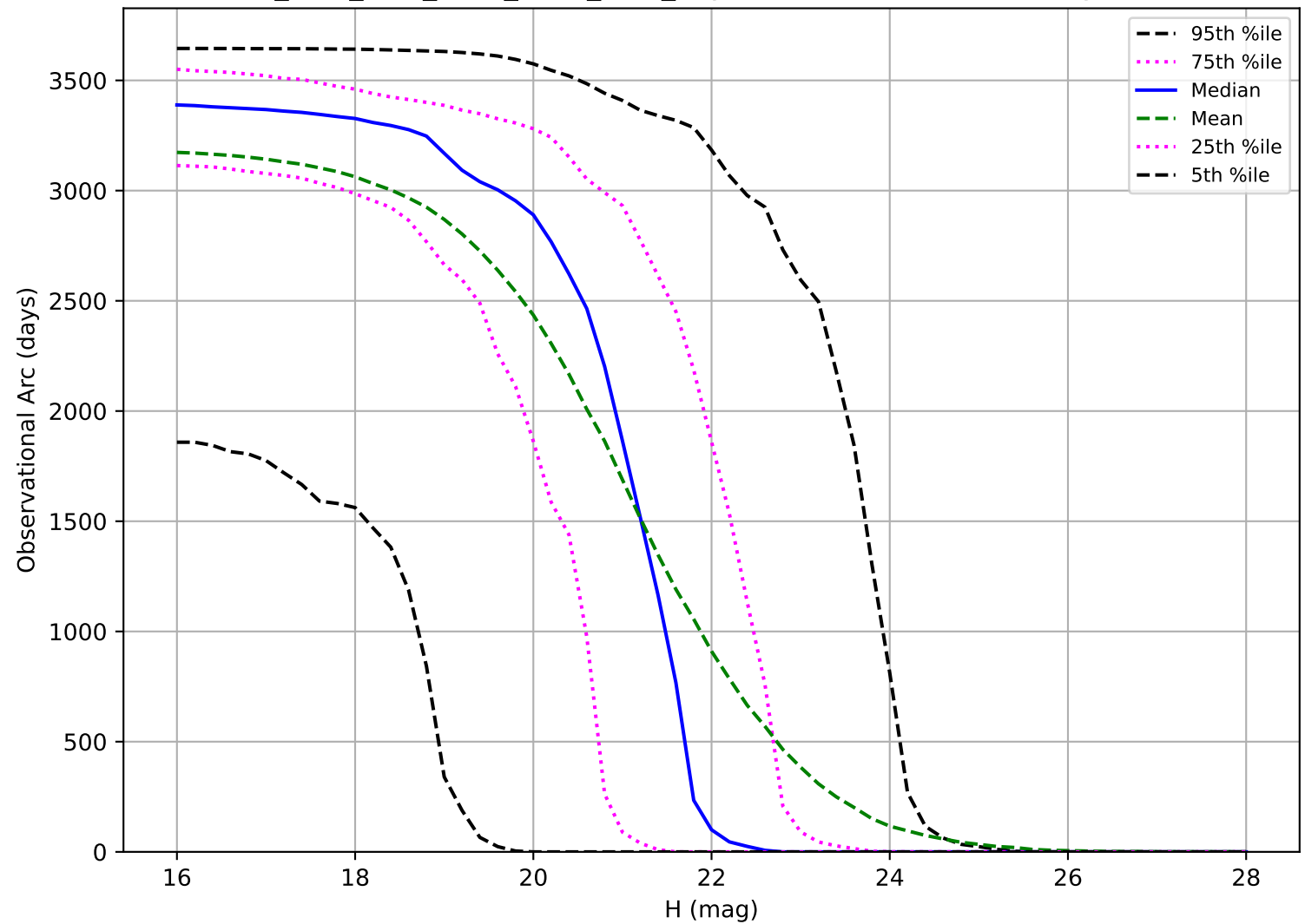
ddf_acor_sf10_lsf20_lsr20_v3.4_10yrs: Observational Arc Length NEO
