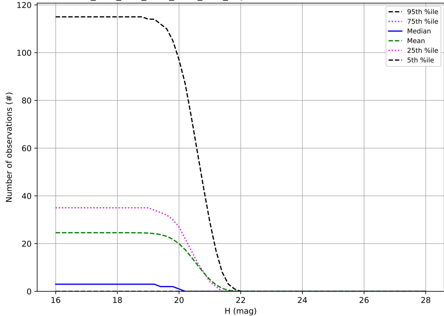
ddf_acor_sf10_lsf20_lsr20_v3.4_10yrs: Number of observations Vatira
