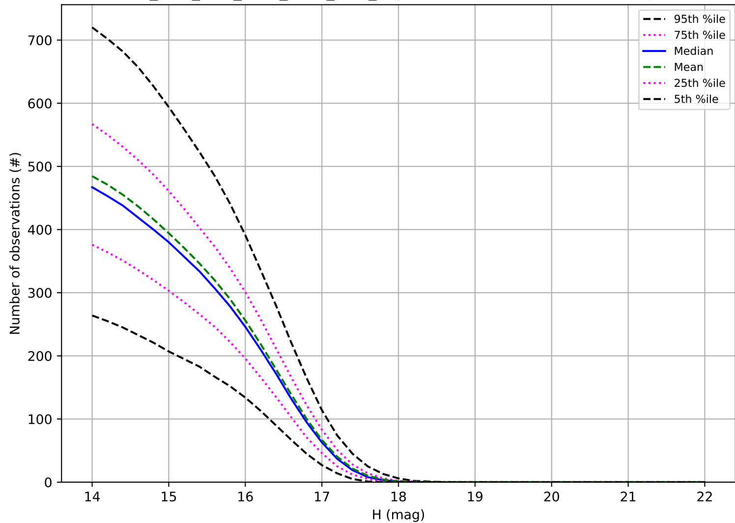
ddf_acor_sf10_lsf20_lsr20_v3.4_10yrs: Number of observations Trojan
