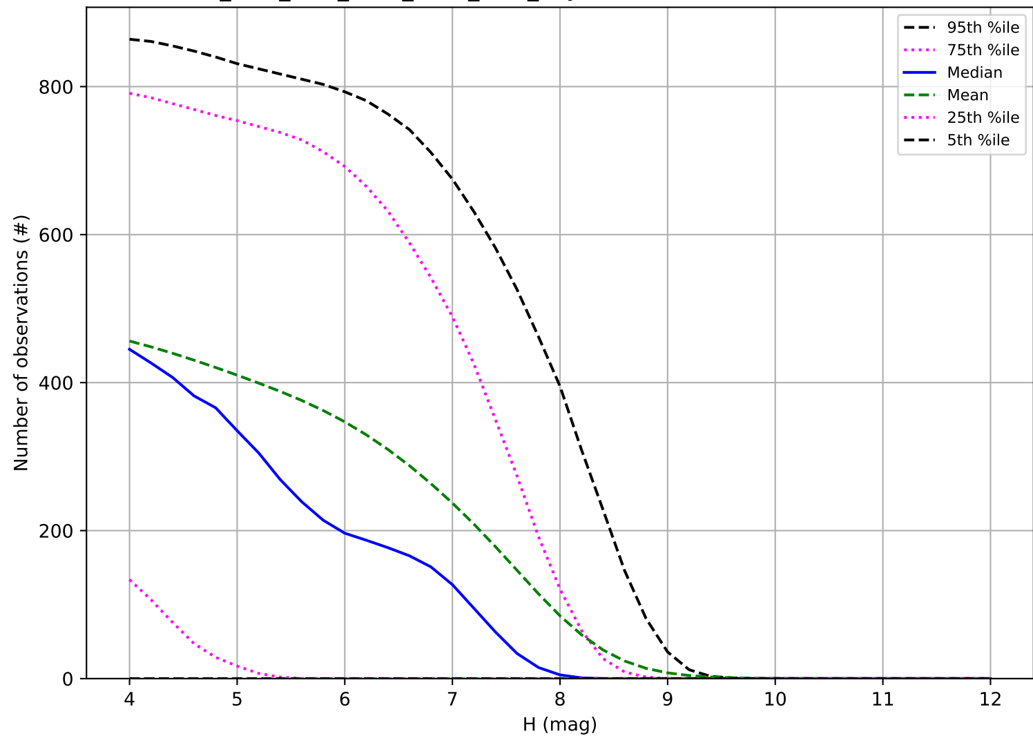
ddf_acor_sf10_lsf20_lsr20_v3.4_10yrs: Number of observations TNO
