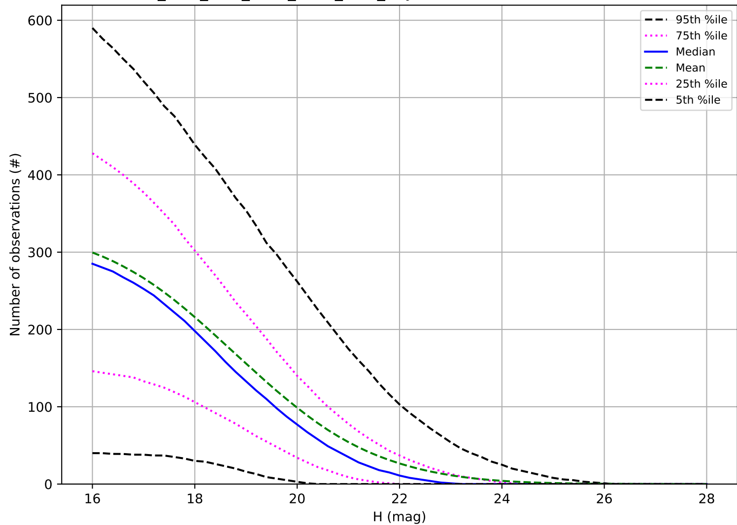
ddf_acor_sf10_lsf20_lsr20_v3.4_10yrs: Number of observations PHA
