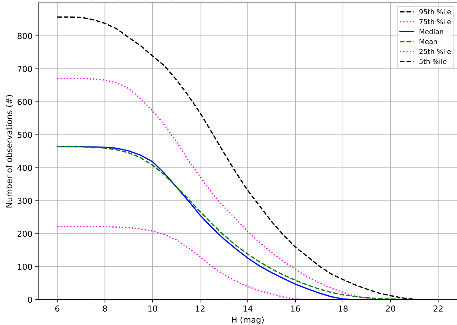
ddf_acor_sf10_lsf20_lsr20_v3.4_10yrs: Number of observations OCC_r5
