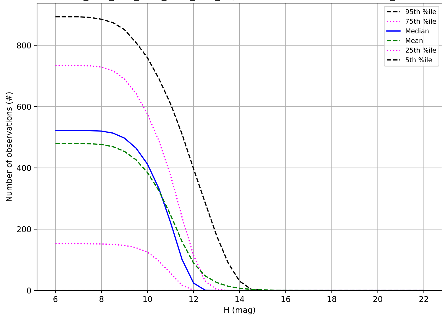
ddf_acor_sf10_lsf20_lsr20_v3.4_10yrs: Number of observations OCC_r20
