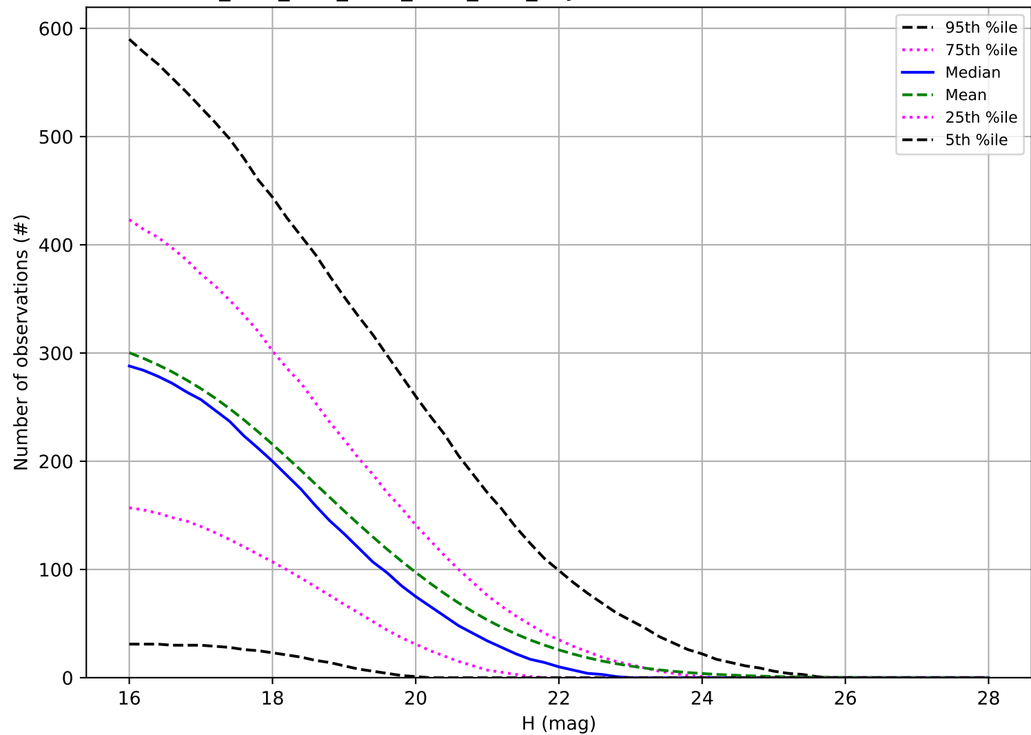
ddf_acor_sf10_lsf20_lsr20_v3.4_10yrs: Number of observations NEO
