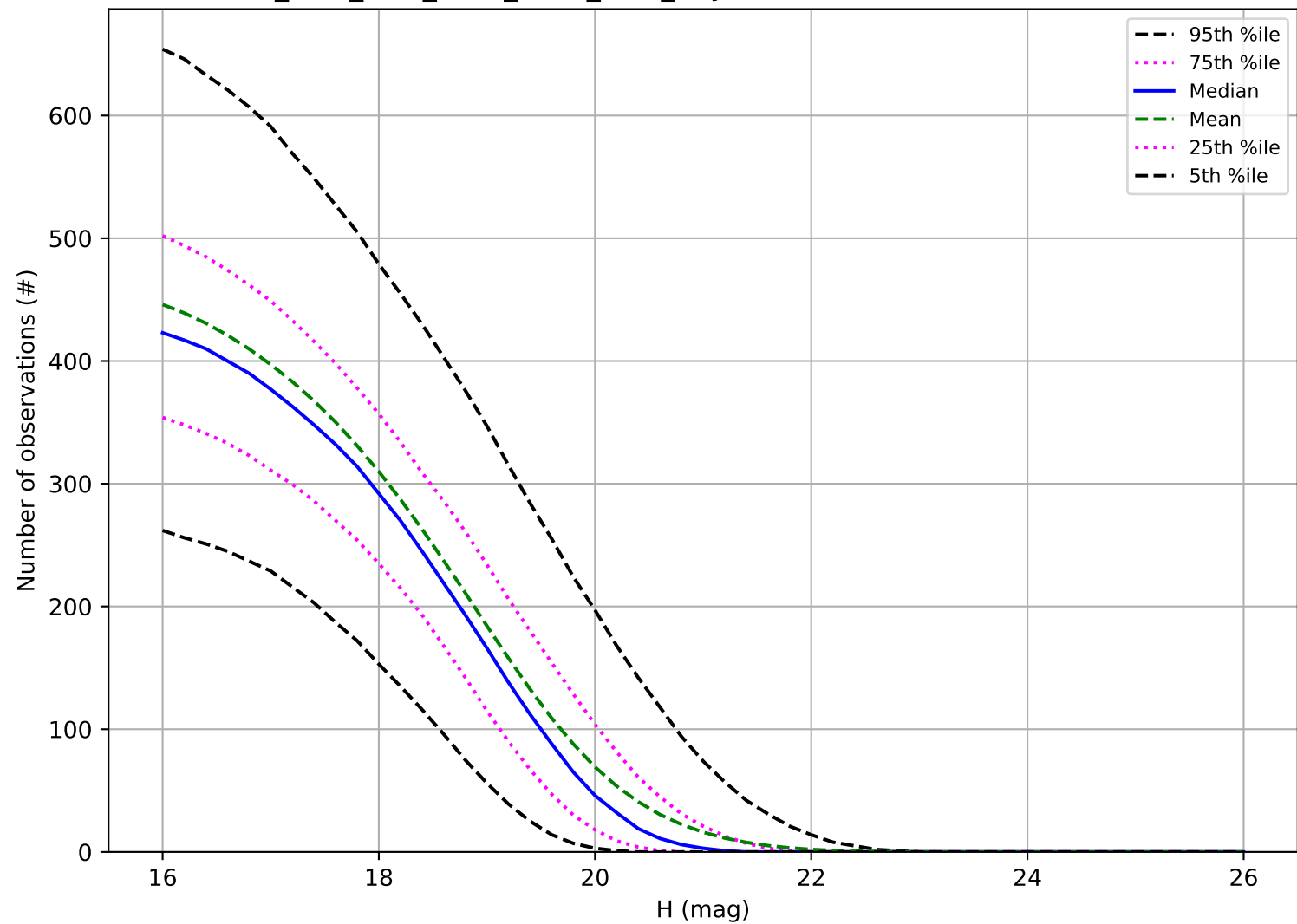
ddf_acor_sf10_lsf20_lsr20_v3.4_10yrs: Number of observations MBA
