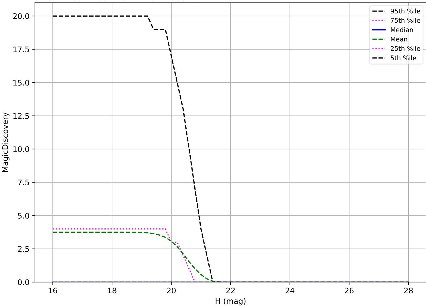
ddf_acor_sf10_lsf20_lsr20_v3.4_10yrs: Vatira 6 detections in 60 nights detection loss
