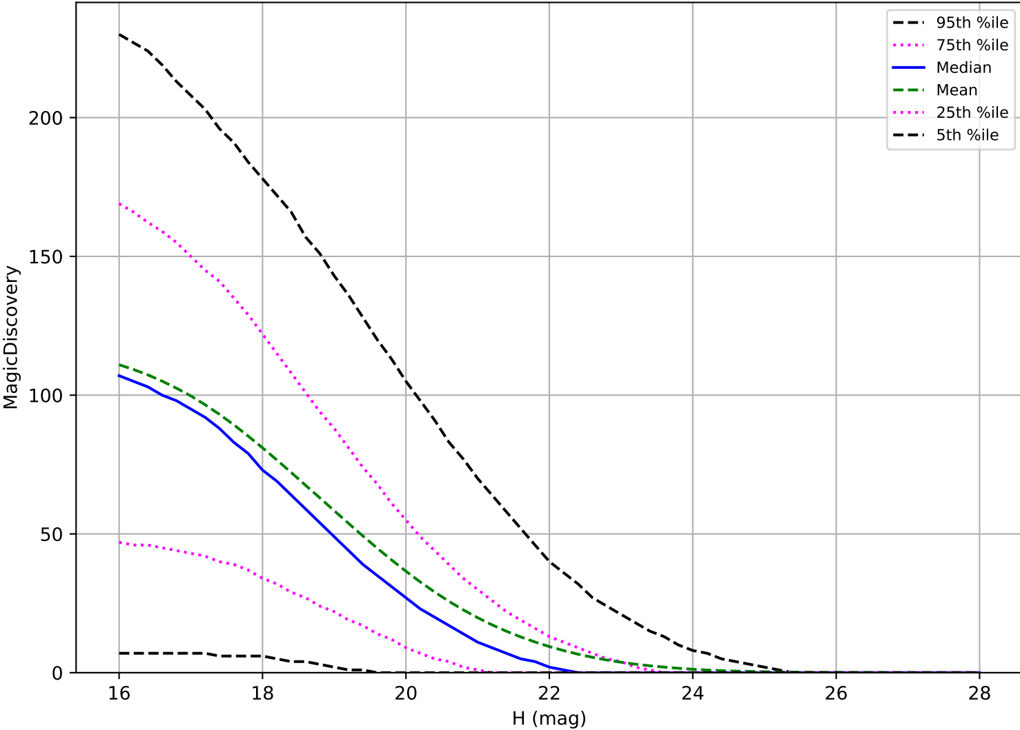
ddf_acor_sf10_lsf20_lsr20_v3.4_10yrs: PHA 6 detections in 60 nights detection loss
