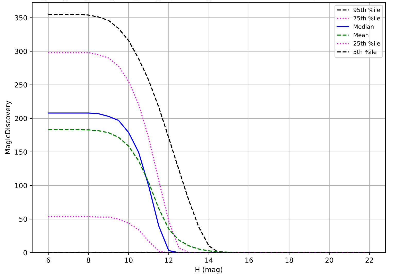
ddf_acor_sf10_lsf20_lsr20_v3.4_10yrs: OCC_r20 6 detections in 60 nights detection loss
