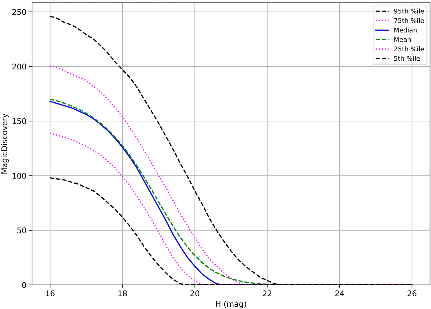
ddf_acor_sf10_lsf20_lsr20_v3.4_10yrs: MBA 6 detections in 60 nights detection loss
