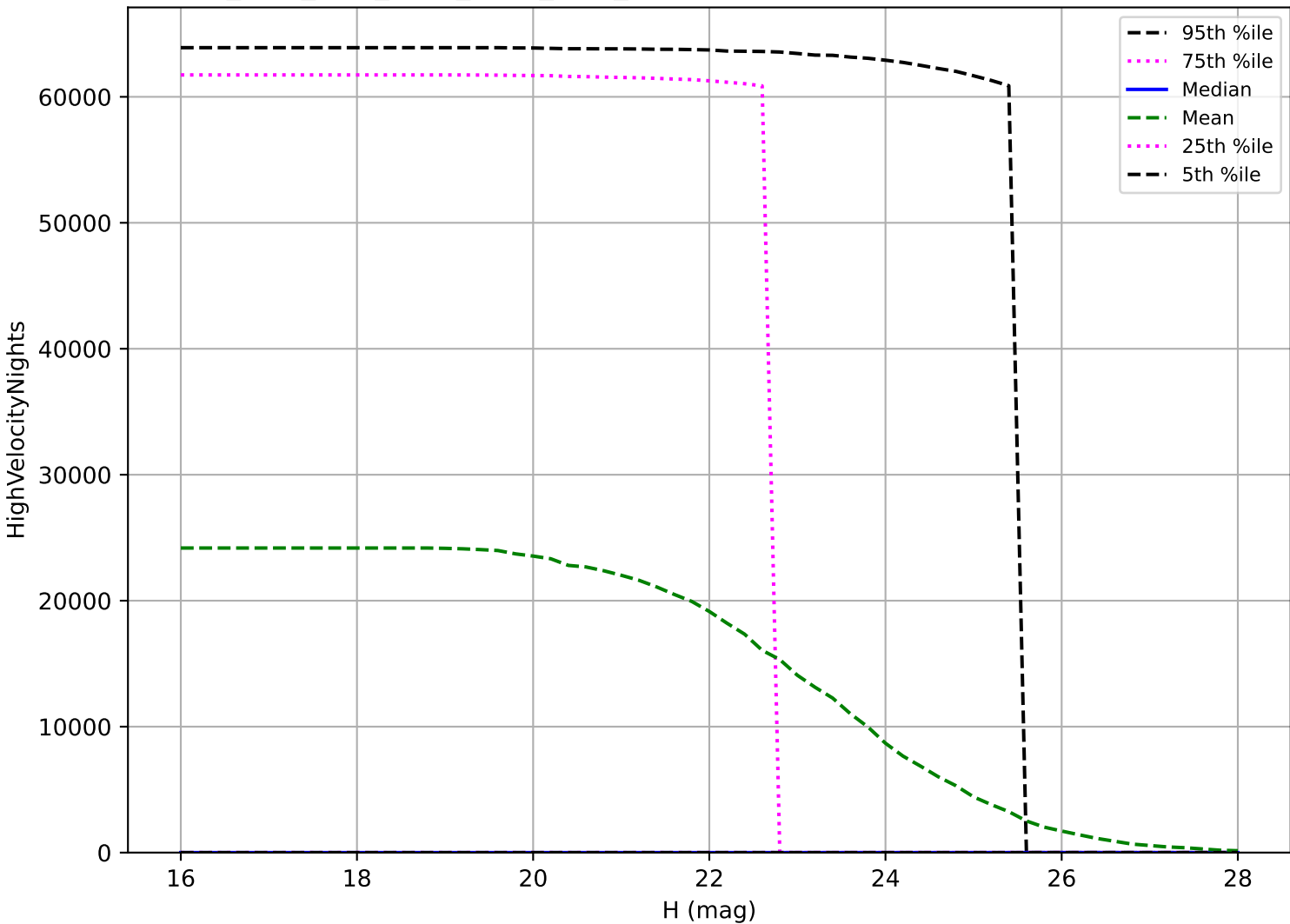
ddf_acor_sf10_lsf20_lsr20_v3.4_10yrs: PHA High velocity pair detection loss
