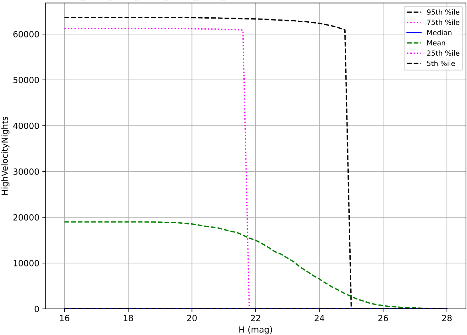
ddf_acor_sf10_lsf20_lsr20_v3.4_10yrs: NEO High velocity pair detection loss
