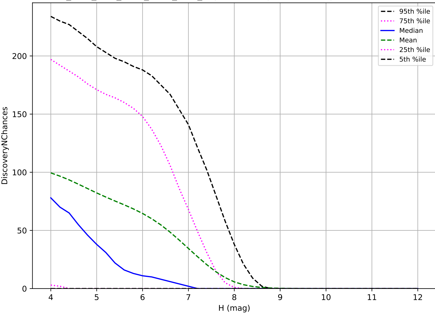
ddf_acor_sf10_lsf20_lsr20_v3.4_10yrs: TNO 3 pairs in 15 nights detection loss
