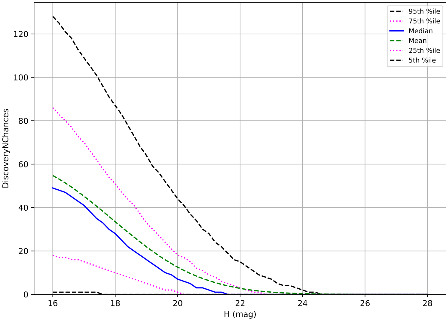
ddf_acor_sf10_lsf20_lsr20_v3.4_10yrs: PHA 3 pairs in 15 nights detection loss
