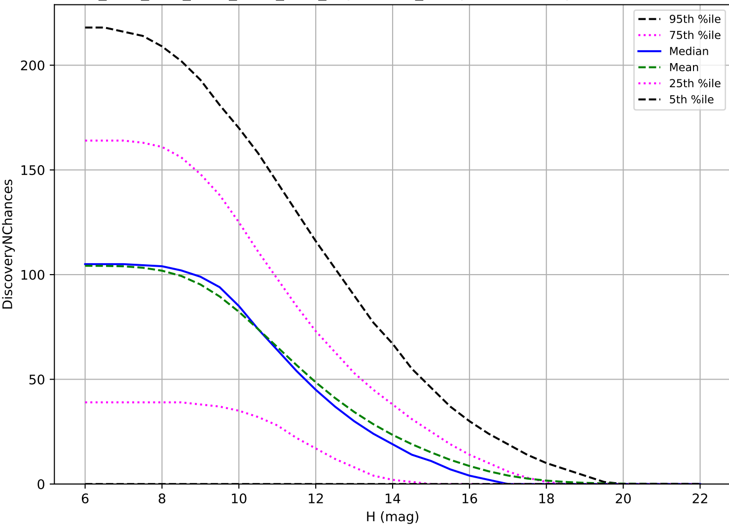
ddf_acor_sf10_lsf20_lsr20_v3.4_10yrs: OCC_r5 3 pairs in 15 nights detection loss
