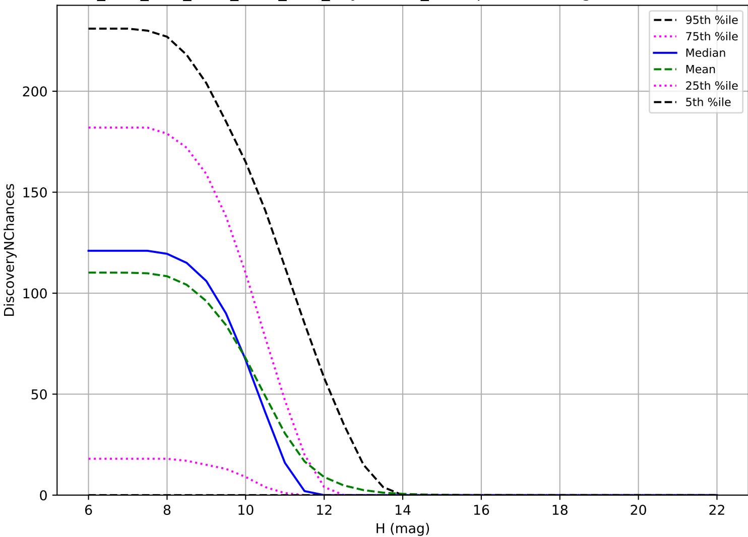
ddf_acor_sf10_lsf20_lsr20_v3.4_10yrs: OCC_r20 3 pairs in 15 nights detection loss
