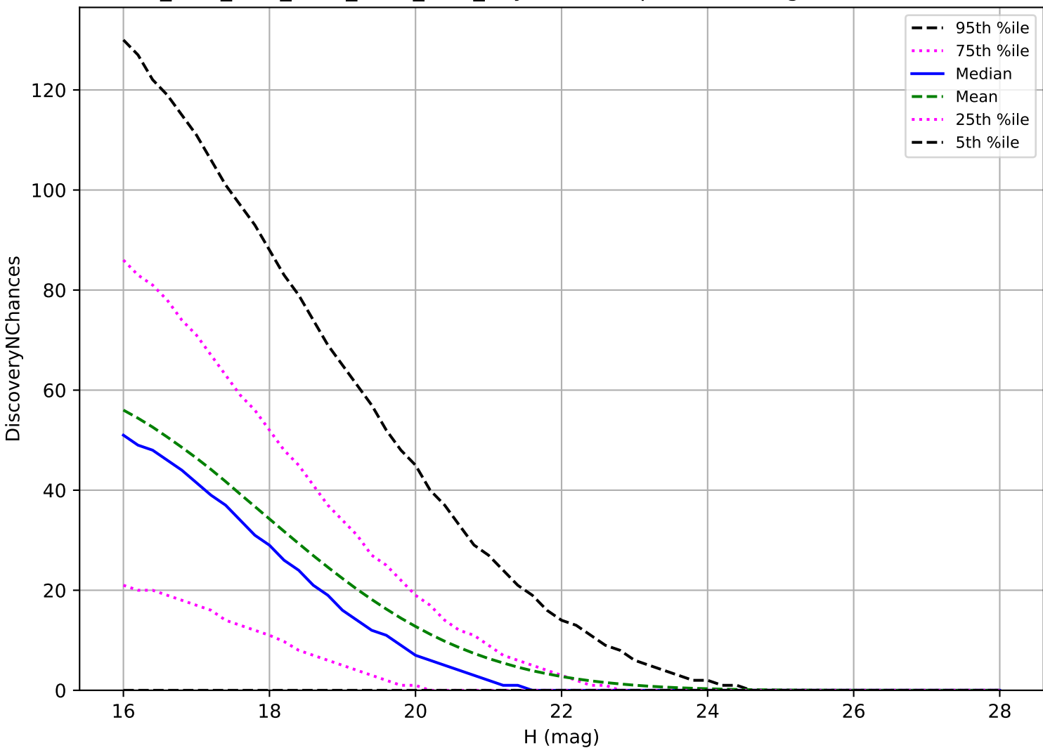
ddf_acor_sf10_lsf20_lsr20_v3.4_10yrs: NEO 3 pairs in 15 nights detection loss
