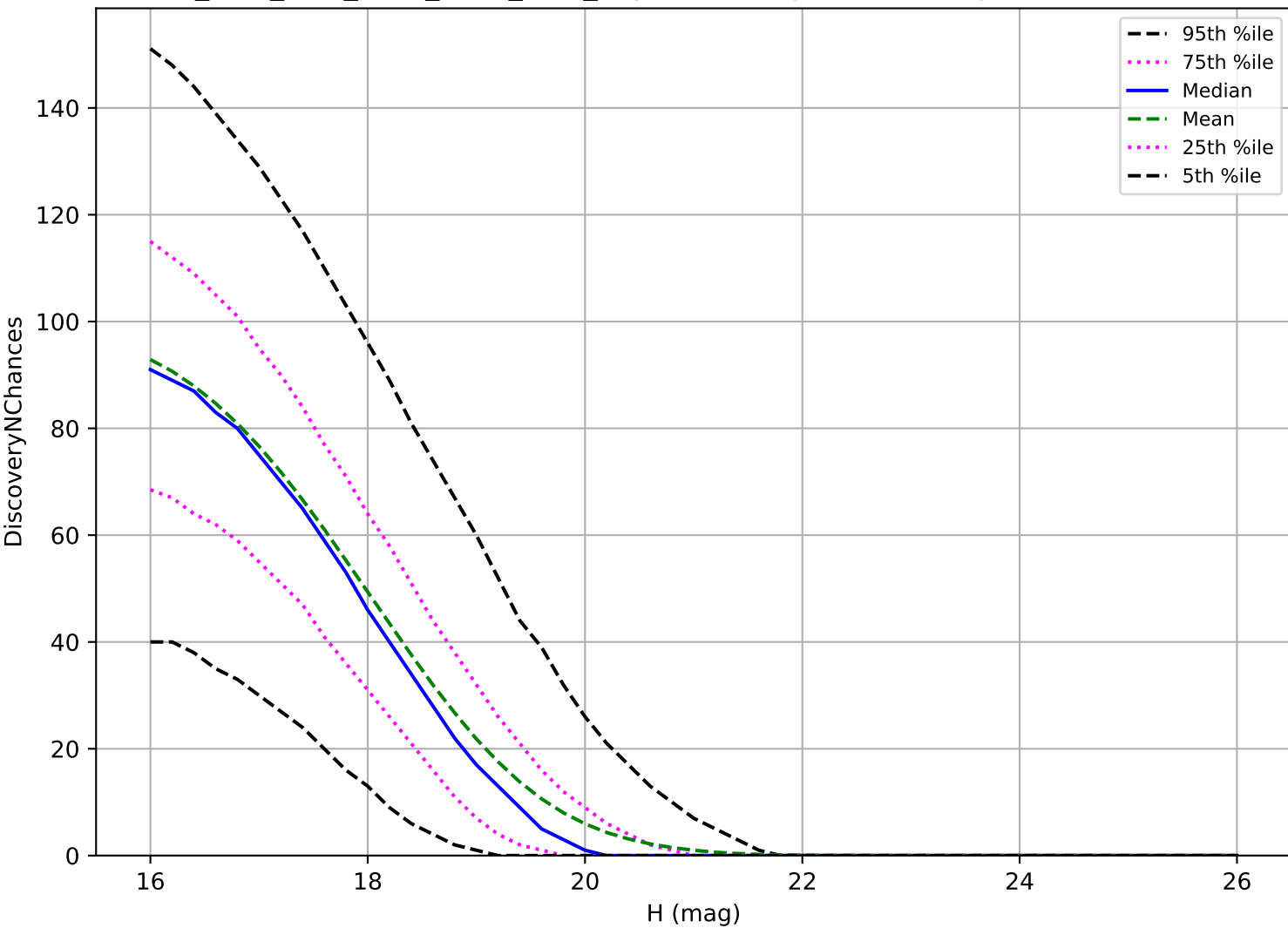
ddf_acor_sf10_lsf20_lsr20_v3.4_10yrs: MBA 3 pairs in 15 nights detection loss
