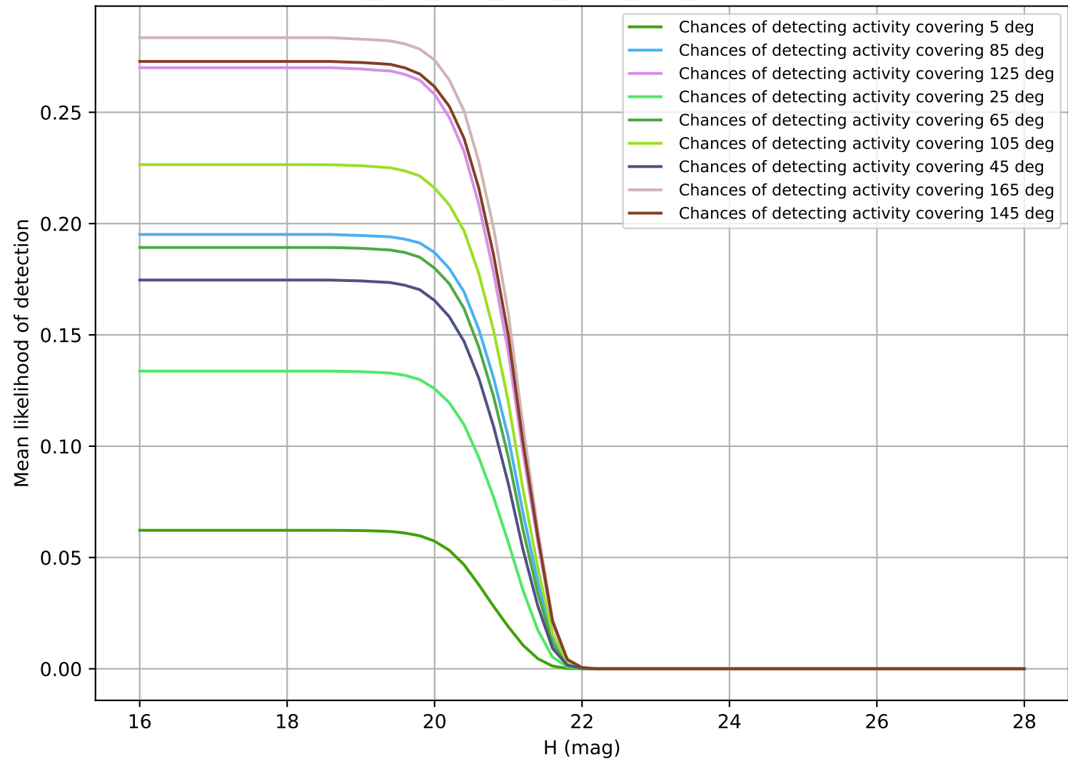
ddf_acor_sf10_lsf20_lsr20_v3.4_10yrs Vatira
