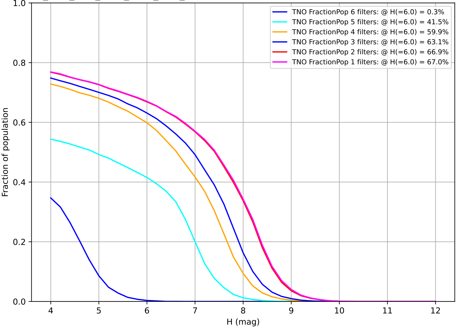
ddf_acor_sf10_lsf20_lsr20_v3.4_10yrs: Fraction of population with colors in X filters TNO
