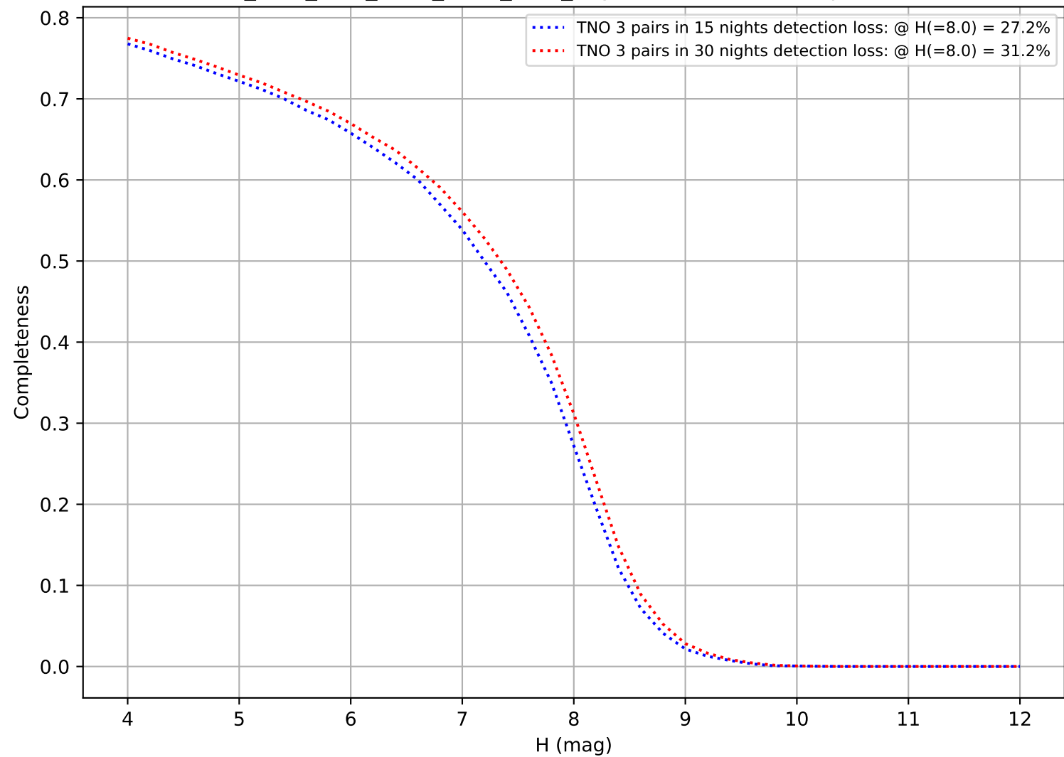
ddf_acor_sf10_lsf20_lsr20_v3.4_10yrs: DifferentialCompleteness
