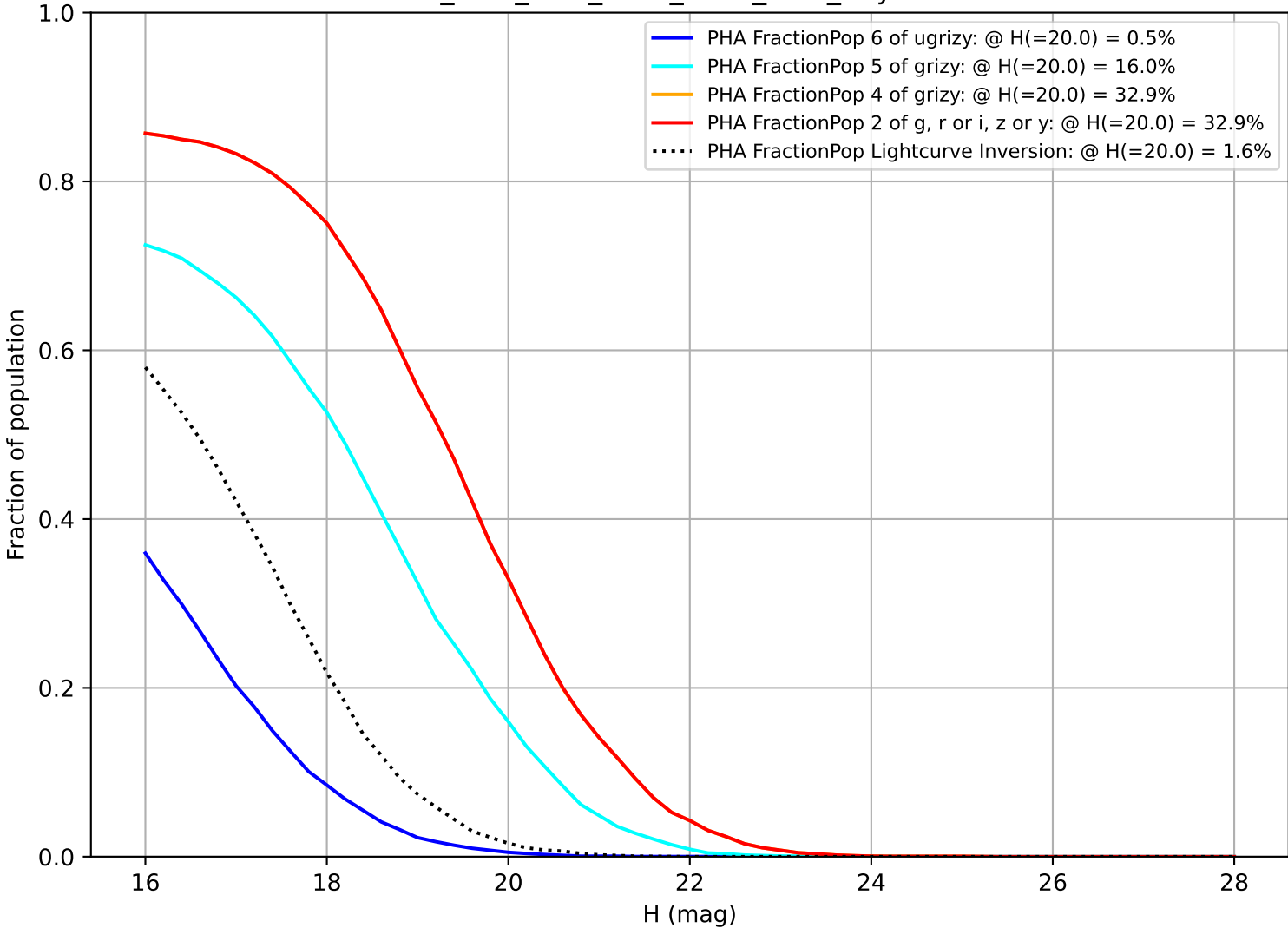
ddf_acor_sf10_lsf20_lsr20_v3.4_10yrs PHA
