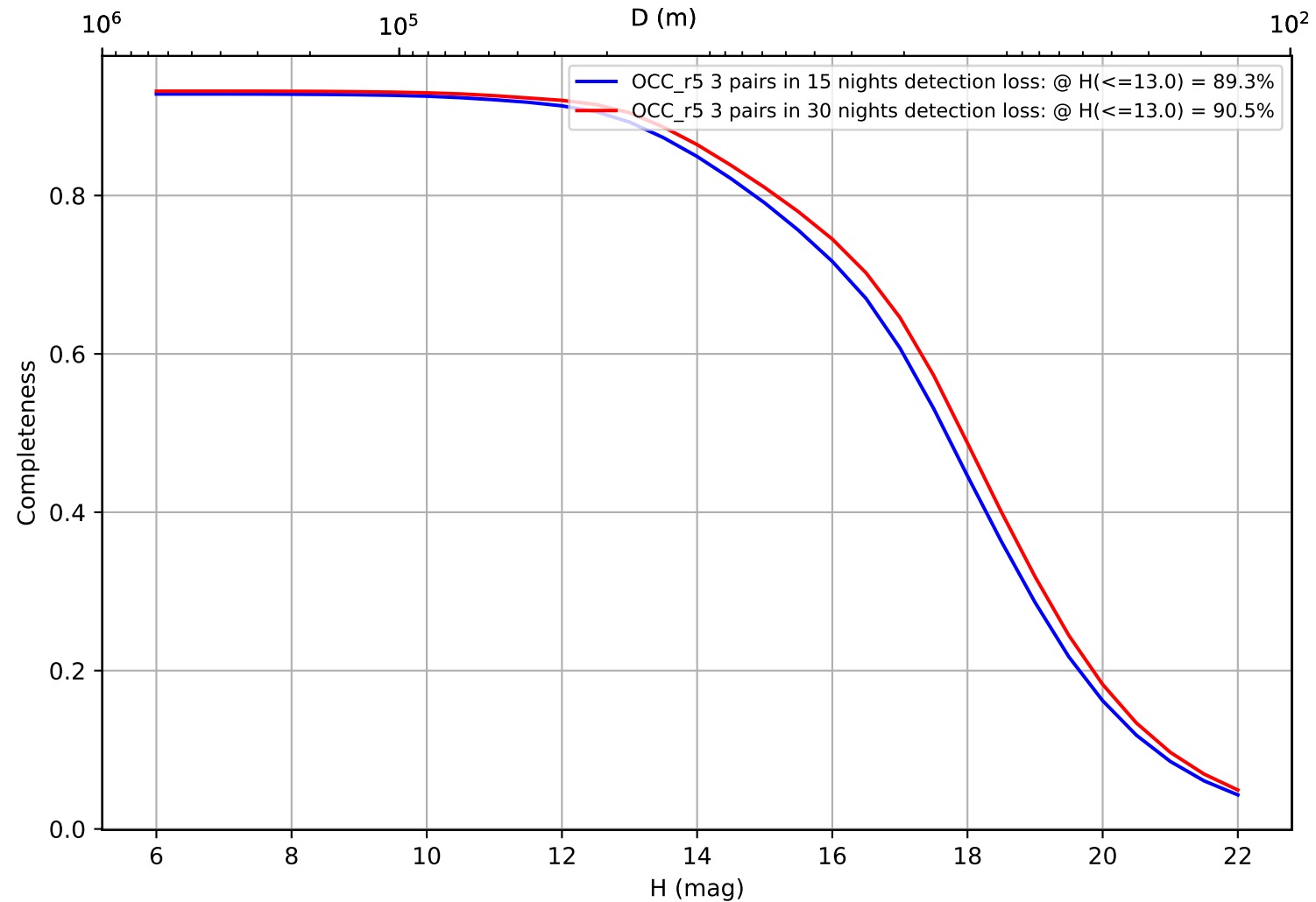
ddf_acor_sf10_lsf20_lsr20_v3.4_10yrs: CumulativeCompleteness
