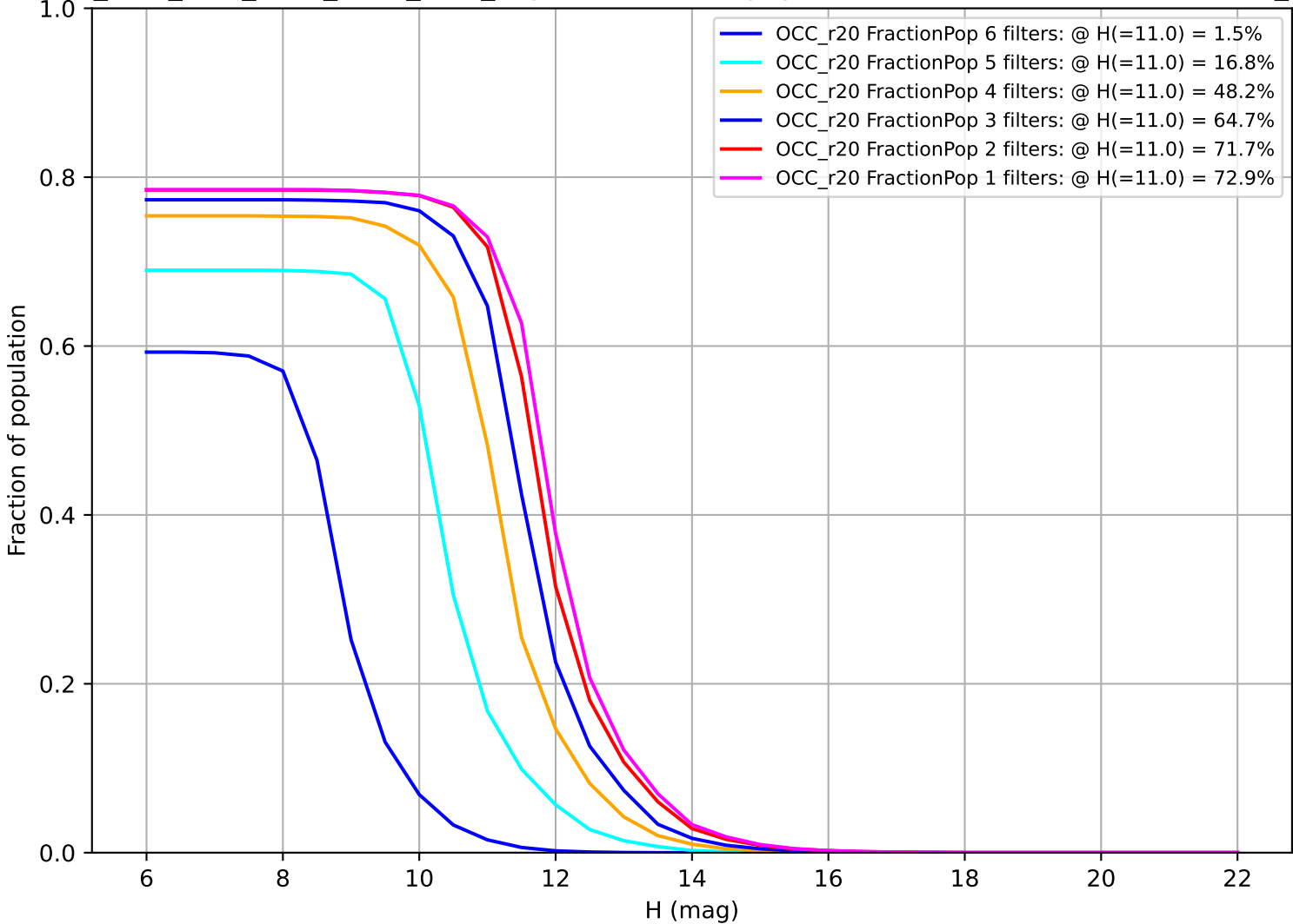
ddf_acor_sf10_lsf20_lsr20_v3.4_10yrs: Fraction of population with colors in X filters OCC_r20
