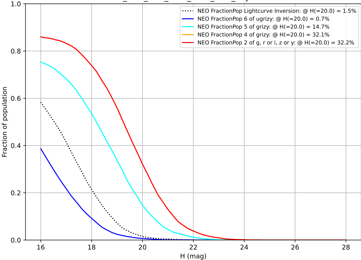
ddf_acor_sf10_lsf20_lsr20_v3.4_10yrs NEO
