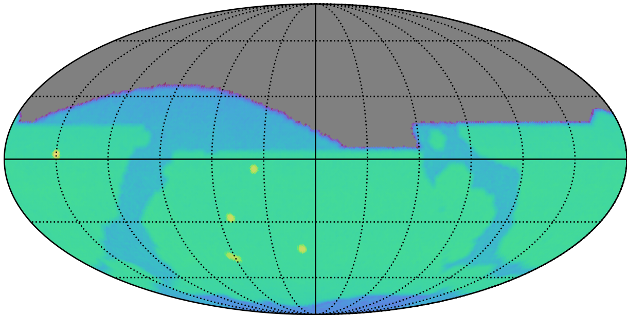
ddf_acor_sf10_lsf20_lsr20_v3.4_10yrs i: SurfaceBrightLimit
