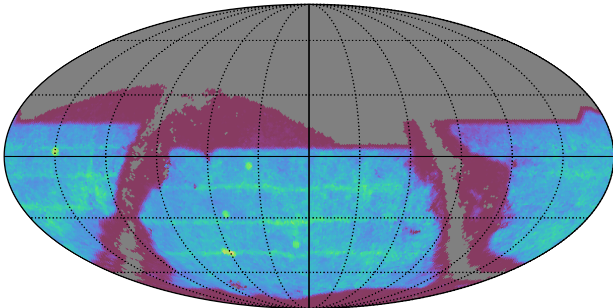
ddf_acor_sf10_lsf20_lsr20_v3.4_10yrs : SNSLMetric
