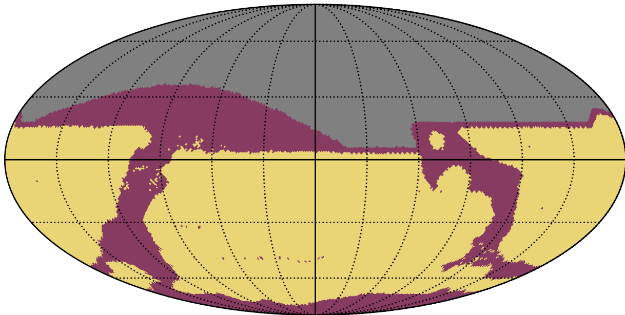
ddf_acor_sf10_lsf20_lsr20_v3.4_10yrs : RapidRevisits
